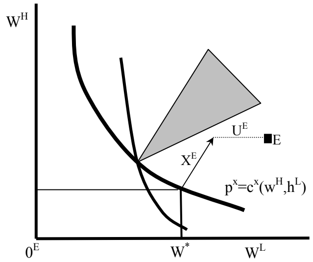
Figure 2 - European Equilibrium
