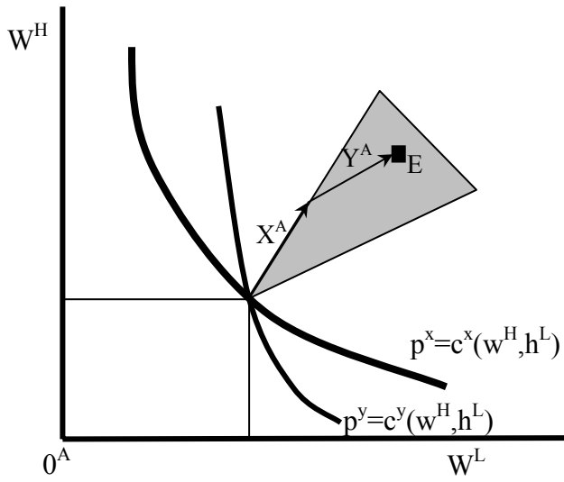
Figure 1- American Equilibrium
